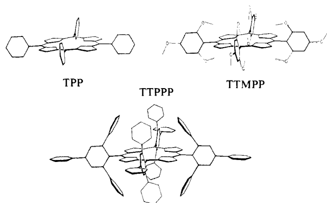
Figure 1. Diagrammatic representations of the porphyrins used in this study.
