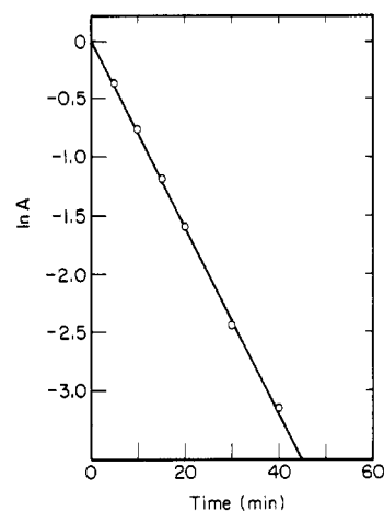
Figure 2. First-order kinetics of the sonolysis of \text{Fe}(\text{CO})_5 . Absorbance at 1999 \text{cm}^{-1} utilized. The observed rate constant in decalin at 21 °C is 1.34 \times 10^{-3} \text{ s}^{-1} ; \tau_{1/2} = 8.6 \text{ min} .
