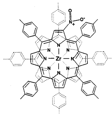
Figure 2. Schematic representation of Zr(TTP)(TTP-NO 2 ), illustrating the proximity of the nitro substituent to two of the p -tolyl groups.
