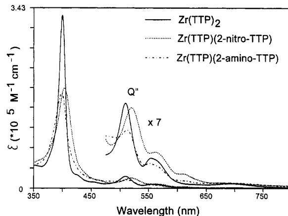
Figure 1. UV-visible spectra of Zr(\text{TPP})(\text{TPP-X}) ( X = \text{H}, \text{NO}_2, \text{NH}_2 ) in toluene.
